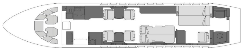
Night Floorplan
