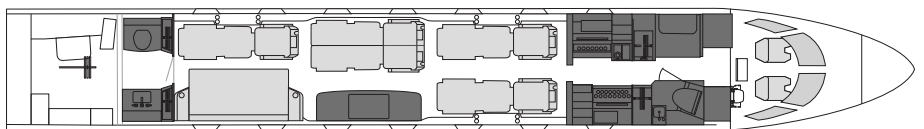
Night Floorplan
